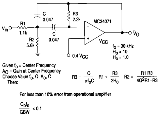
Figure 42. Active Bandpass Filter
