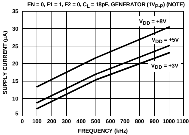
FIGURE 17. DISABLE SUPPLY CURRENT vs FREQUENCY
