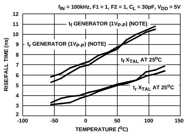
FIGURE 32. RISE/FALL TIME vs TEMPERATURE
