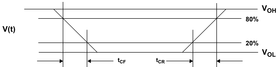
Figure 5. Voltage Waveforms
