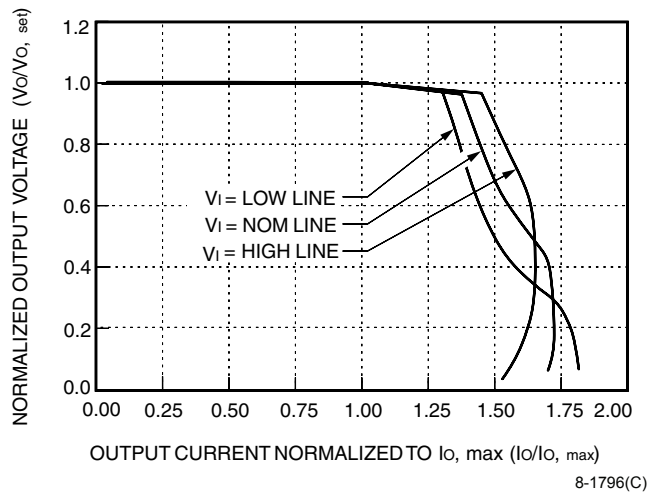
Figure 12. Lx010x/Lx015x Single-Output Normalized Output Current vs. Normalized Output Voltage at T_c = 25\text{ }^{\circ}\text{C}
