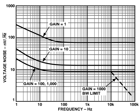
Figure 8. Voltage Noise Spectral Density vs. Frequency, ( G = 1\text{--}1000 )
