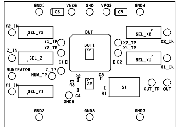
Figure 30. AD633-EVALZ Assembly
