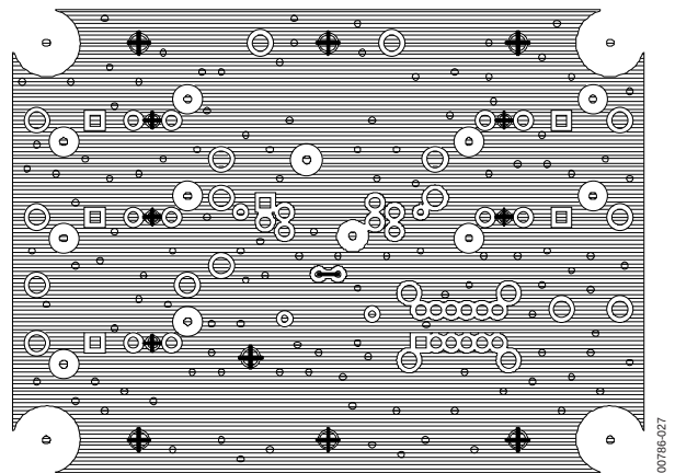
Figure 26. Circuit Side Copper
