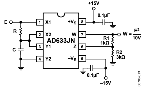
Figure 14. Bounceless Frequency Doubler
