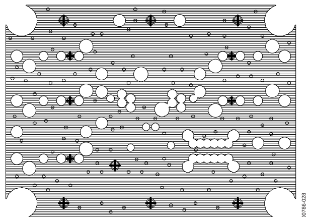
Figure 27. Inner Layer Ground Plane
