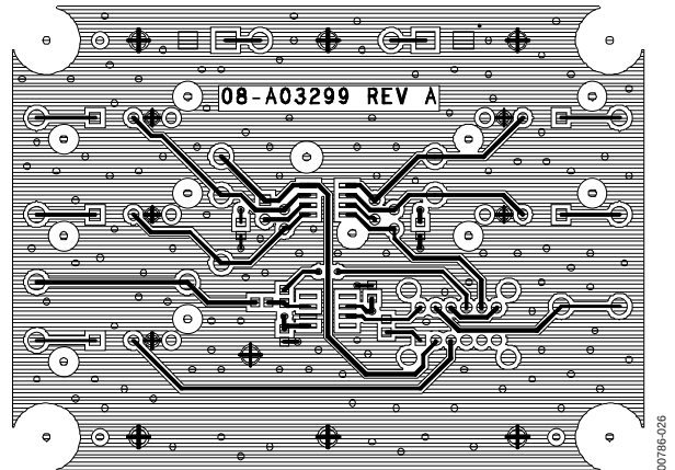
Figure 25. Component Side Copper
