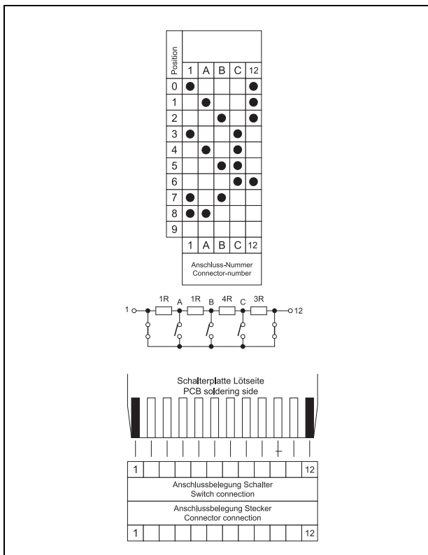
Code 632 Resistance decade
