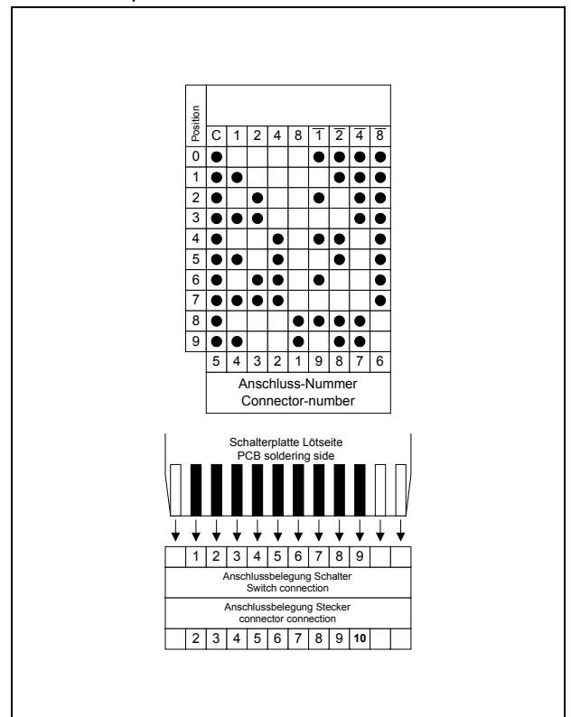
Code 531 BCD + complement
