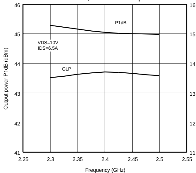
P1dB, GLP vs. Freq.
