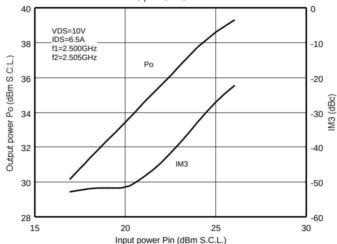
Po, IM3 vs. Pin
