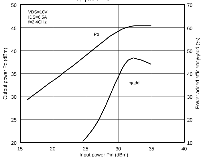
Po, \eta_{add} vs. Pin
