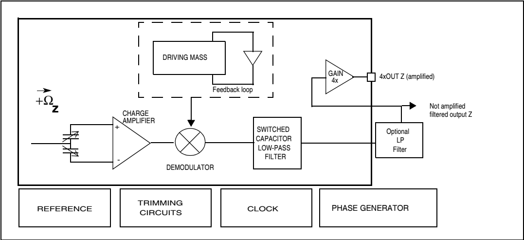
Figure 1. Block diagram
