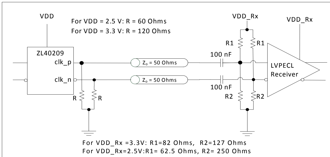
Figure 17 - LVPECL AC Output Termination
