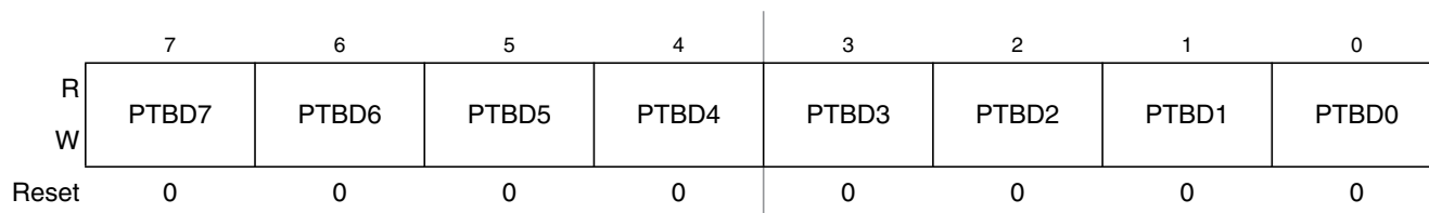
Figure 6-14. Port B Data Register (PTBD)
