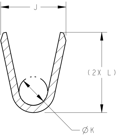
SECTION AF-AF SCALE 20:1
