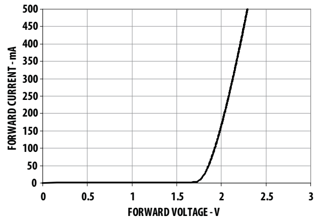
Figure 2. Forward Current vs Forward Voltage for AlInGaP
