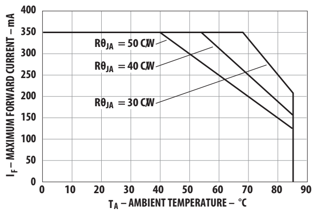
Figure 11. Maximum Forward Current vs. Ambient Temperature for InGaN Derated based on T_{j,MAX} = 110^{\circ}\text{C} , R_{\theta JA} = 30^{\circ}\text{C/W} , 40^{\circ}\text{C/W} and 50^{\circ}\text{C/W}
