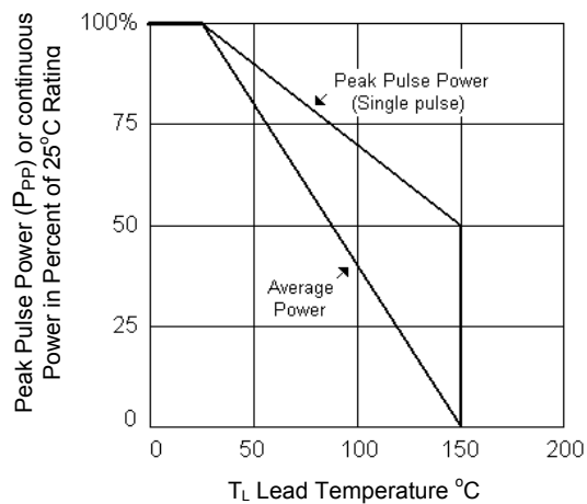
FIGURE 3 Derating Curve
