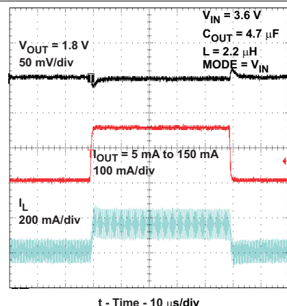
Figure 50. Load Transient Response 5 mA to 150 mA, Forced PWM Mode, V_{OUT} 1.8 V – TPS62231
