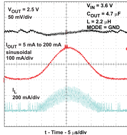
Figure 47. AC – Load Regulation Performance 2.5-V V_{OUT} , PFM Mode – TPS62230
