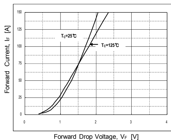
Fig15. Forward characteristics
