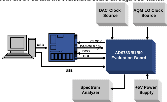
Figure 1- Bench Set-Up
