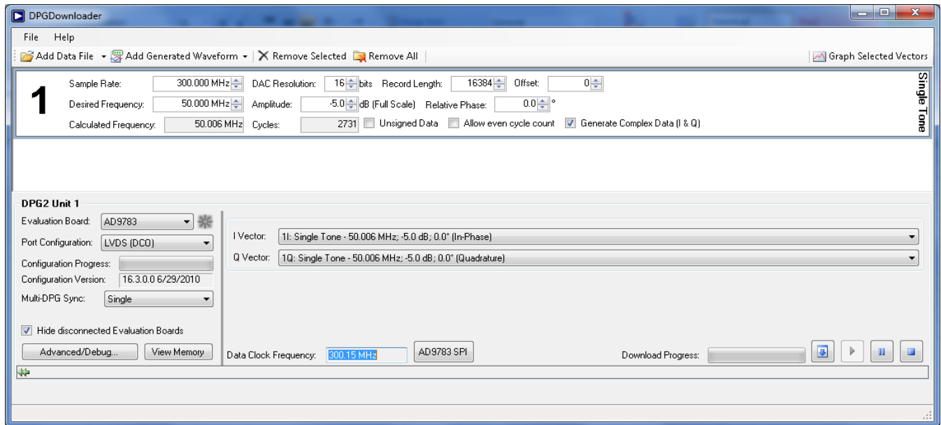
Figure 5 – DPGDownloader Window
