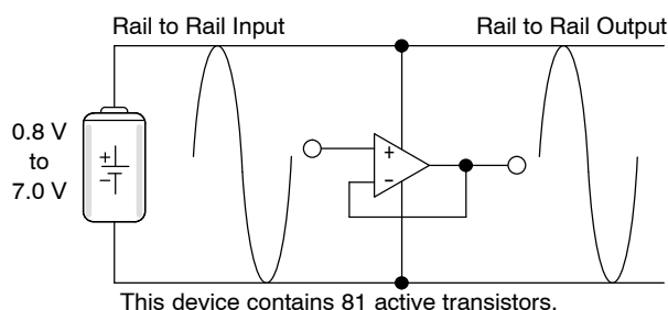
Figure 1. Typical Application
