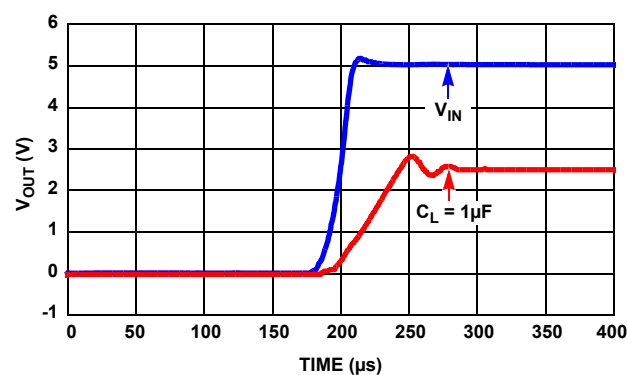
FIGURE 27. TURN-ON TIME WITH 1μF
