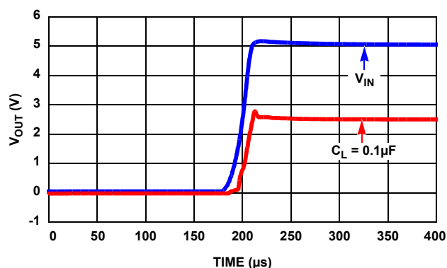
FIGURE 26. TURN-ON TIME WITH 0.1μF
