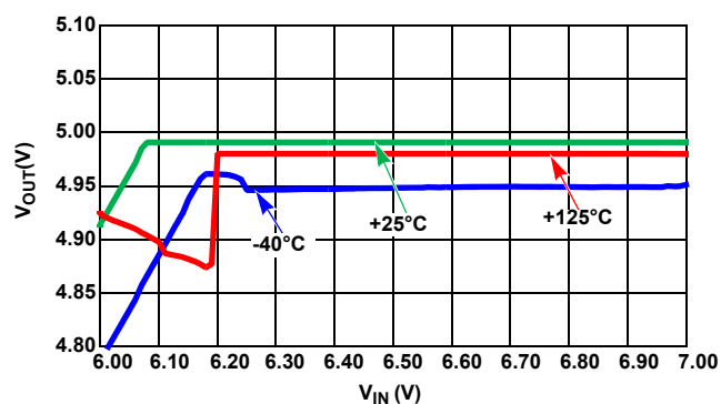
FIGURE 51. DROPOUT WITH -10mA LOAD
