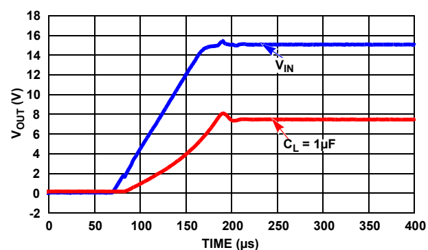
FIGURE 61. TURN-ON TIME WITH 1 \mu\text{F}
