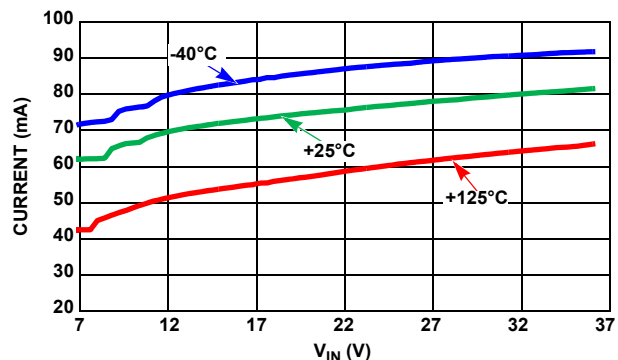
FIGURE 49. SHORT-CIRCUIT TO V IN
