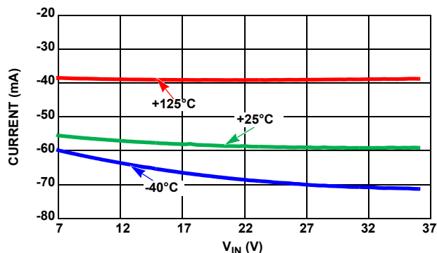
FIGURE 48. SHORT-CIRCUIT TO GND
