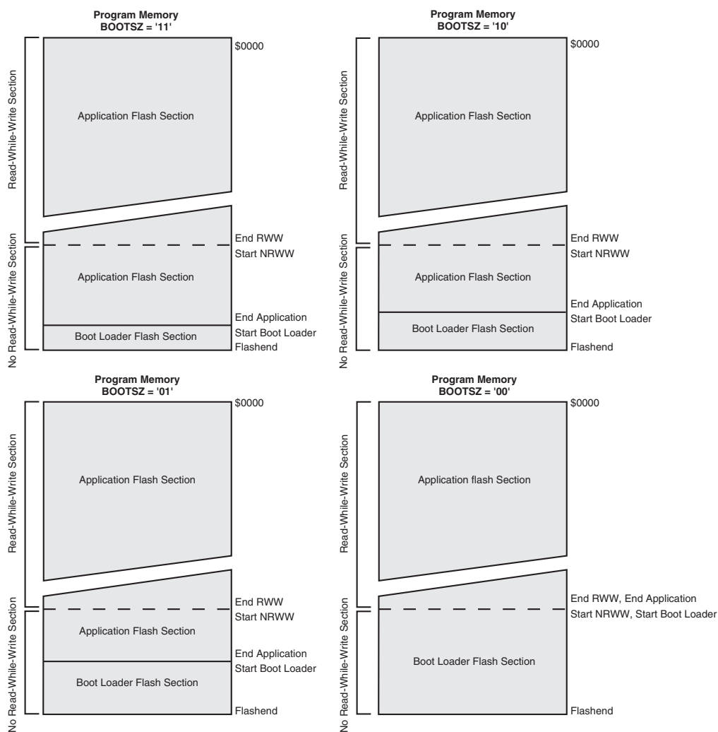
Figure 24-2. Memory Sections (1)
