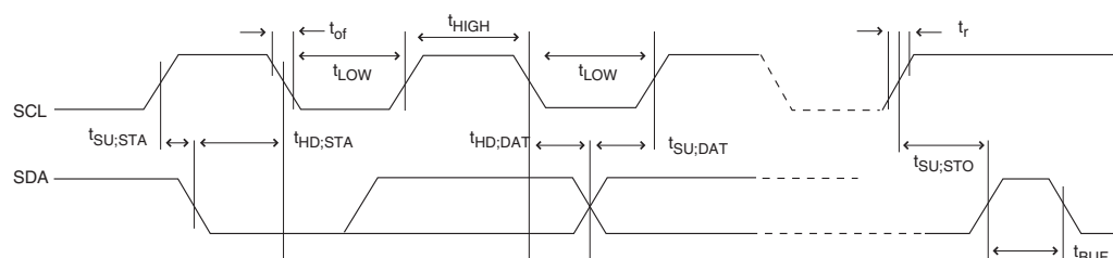
Figure 26-3. Two-wire Serial Bus Timing
