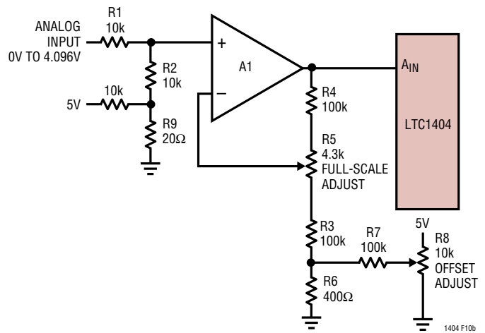
Figure 10b. LTC1404 Offset and Full-Scale Adjust Circuit
