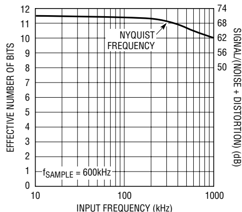
Unipolar Mode ENOB and Signal/(Noise + Distortion) vs Input Frequency
