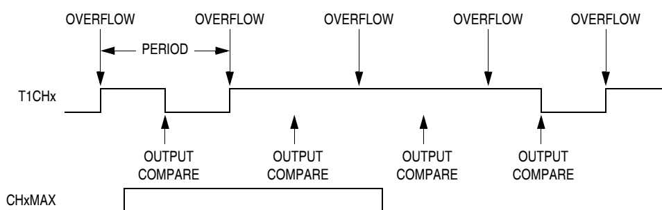
Figure 14-11. CHxMAX Latency
