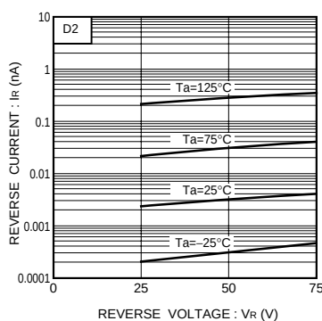
Fig.8 Reverse characteristics
