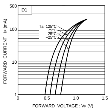
Fig.5 Forward characteristics
