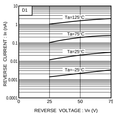
Fig.7 Reverse characteristics
