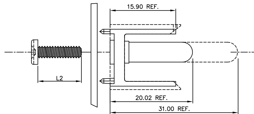
SINGLE GUIDE PIN ASSEMBLY
