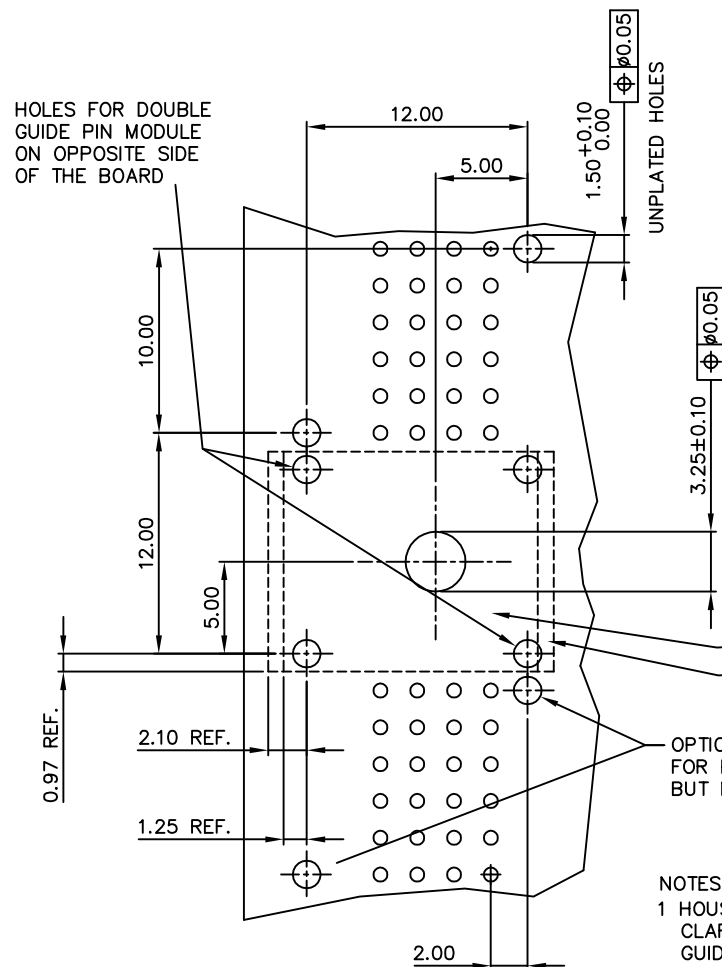
RECOMMENDED HOLE PATTERN COMPONENT SIDE
