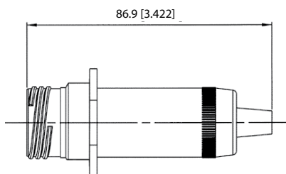
Backshell used with back termination type 1: USB A receptacle Same panel drilling as USBF TV 2xx
