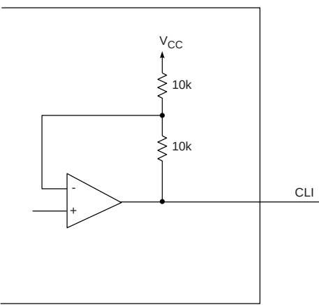
Figure 5 CLI Output Circuit
