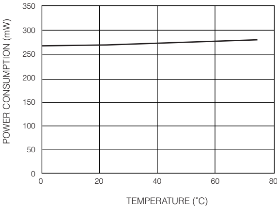
Figure 7 Power Consumption
