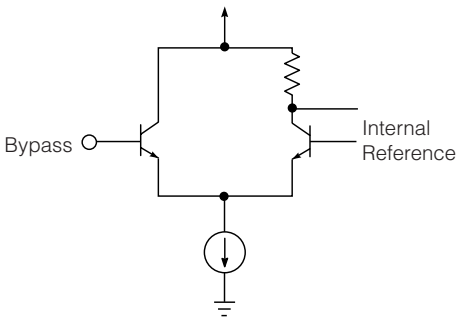
Figure 6 Bypass Circuit
