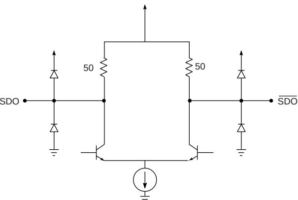
Figure 4 Output Circuit
