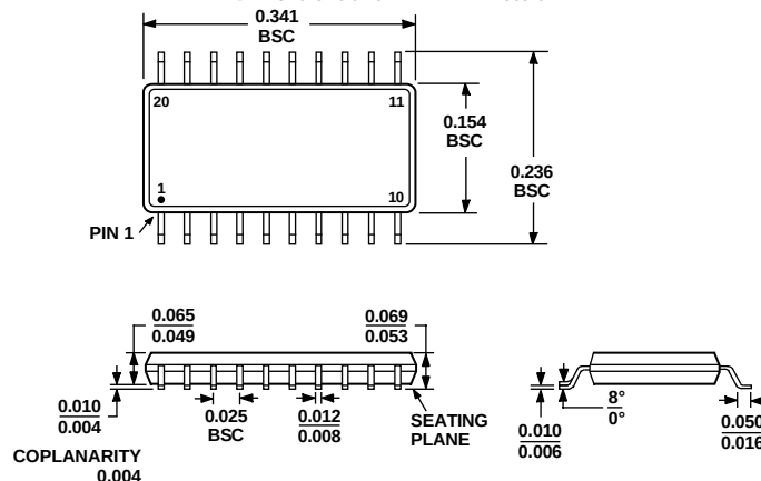
Figure 31. 20-Lead Shrink Small Outline Package [QSOP] (RQ-20)
