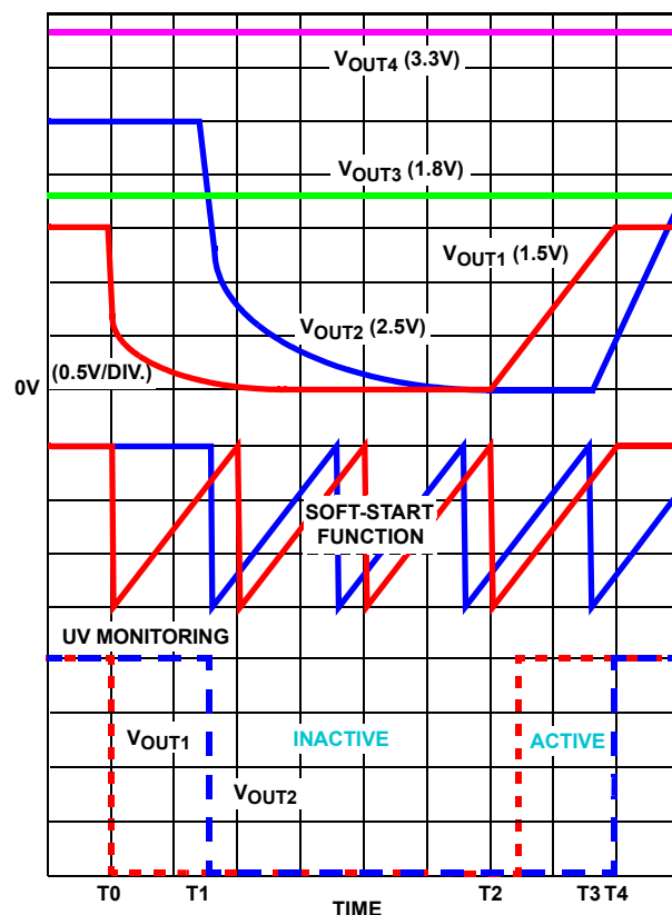
FIGURE 2. OVERCURRENT/UNDERVOLTAGE PROTECTION RESPONSE
