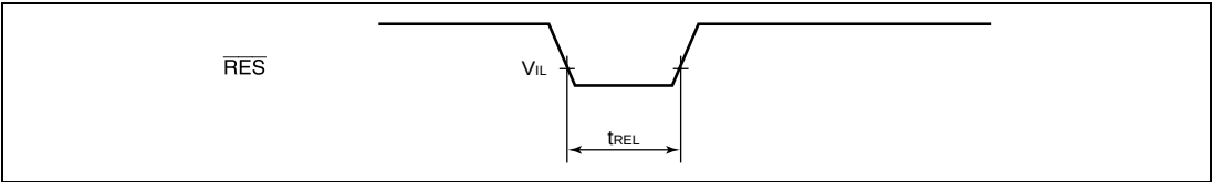
Figure 17.2 \overline{RES} Low Width Timing
