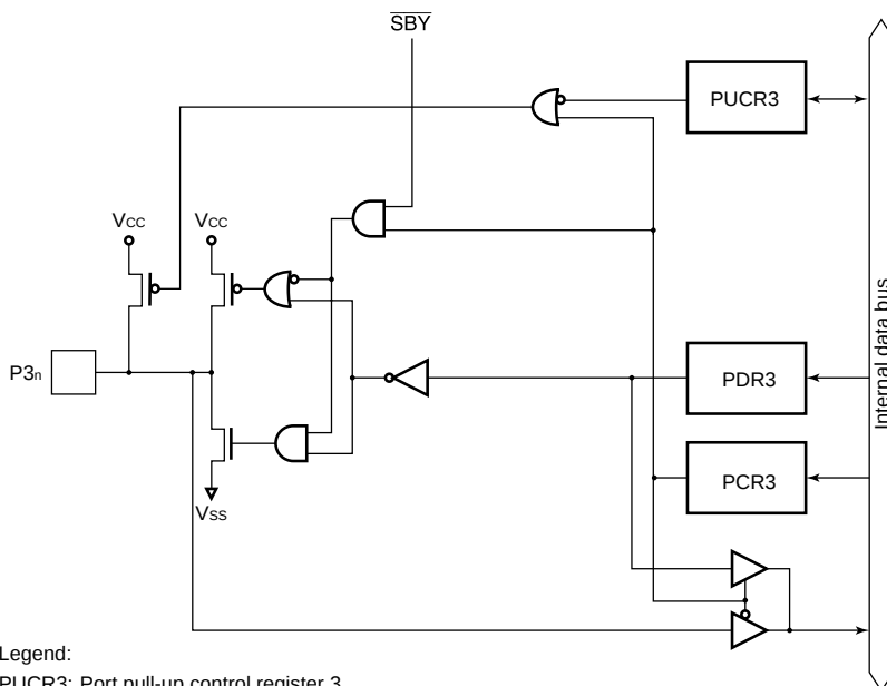
Figure B.1(b) Port 3 Block Diagram (Pin P35)
