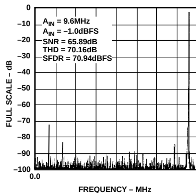
Figure 9. FFT Plot
