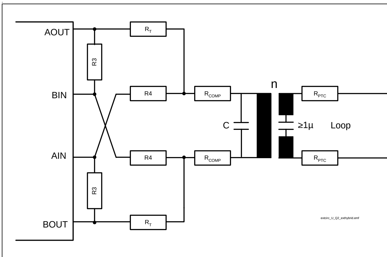
Figure 102 External Circuitry Q- and T-SMINT ® IX
