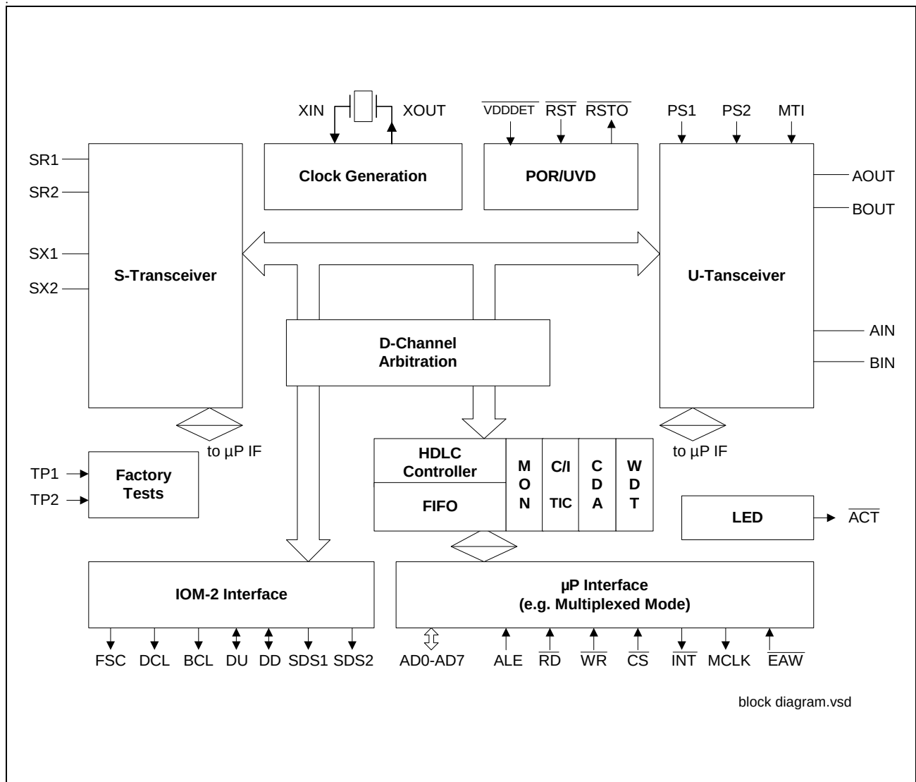
Figure 2 Block Diagram
