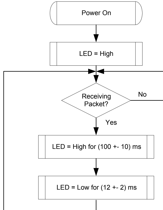
Figure 8. Rx LED
