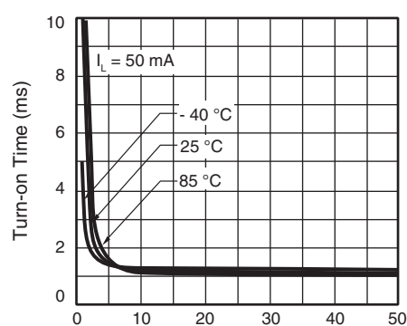
Fig. 18 - Turn-on Time vs. LED Current
