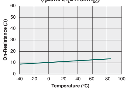
Form-B Typical On-Resistance vs. Temperature ( I_F=5\text{mA} , I_L=170\text{mA}_{\text{DC}} )
