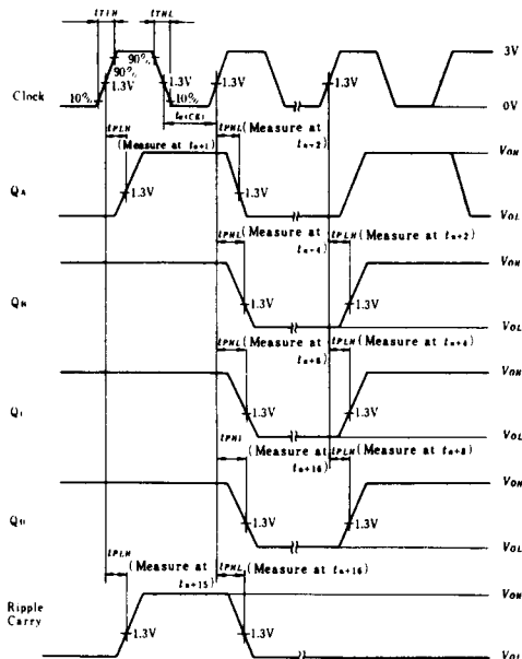
Waveform—1 f_{max} , t_{PLH} , t_{PHL} (Clock→Q, Ripple Carry)
