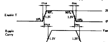
Waveform—3 t_{PLH} , t_{PHL} (Enable T→Ripple Carry)
