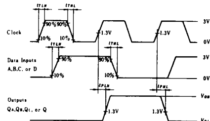
Waveform—2 t_{PLH} , t_{PHL} (Clock→Q)
