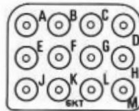
Layout 12 12 Size 20 Contacts
