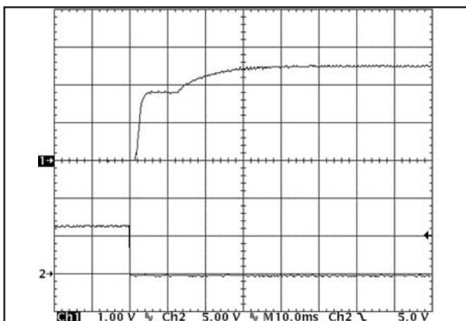
Figure 10: Turn-on transient at zero load (10 ms/div). Top Trace: V out (1V/div) Bottom Trace: ON/OFF input (5V/div)
