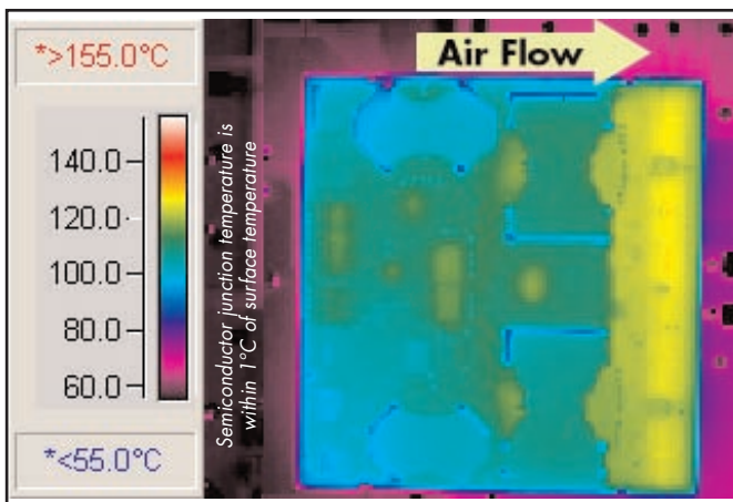
Figure 8: Thermal plot of converter at 48 amp load current with 55°C air flowing at the rate of 200 LFM. Air is flowing across the converter from input to output (nominal input voltage).
