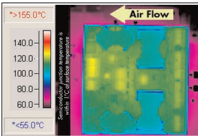
Figure 6: Thermal plot of converter at 50 amp load current with 55°C air flowing at the rate of 200 LFM. Air is flowing across the converter from output to input (nominal input voltage).
