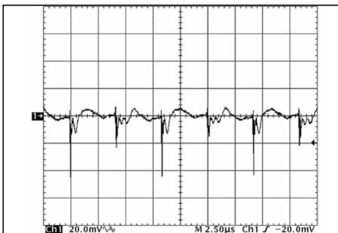
Figure 16: Output voltage ripple at nominal input voltage and rated load current (20 mV/div). Load capacitance: 1\ \mu F ceramic capacitor and 10\ \mu F tantalum capacitor. Bandwidth: 20 MHz. (See Figure 13)
