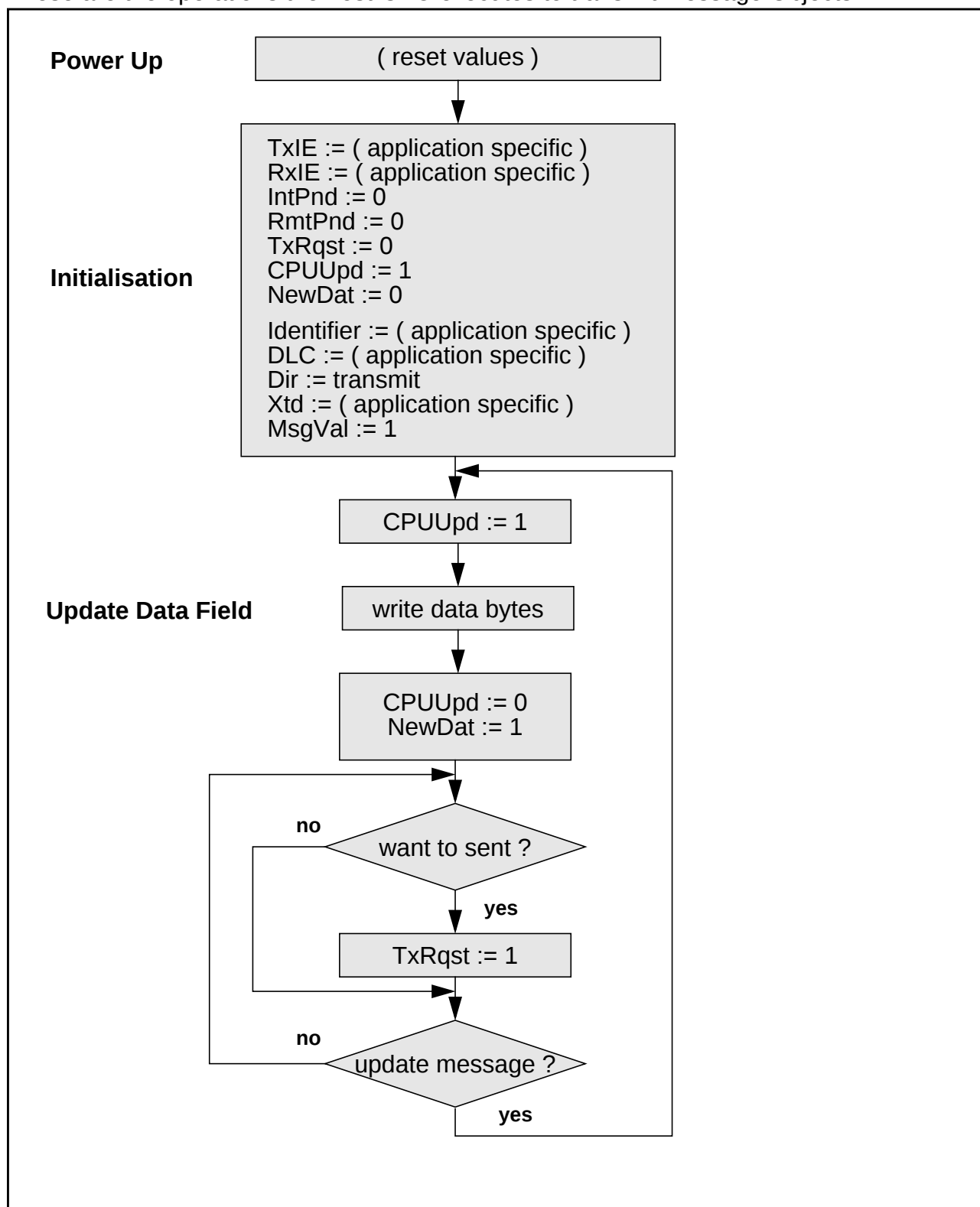
Figure 7: CPU Handling of Message Objects 1-14 (Transmit)
