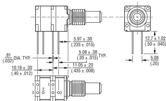
Model 93 PC Pin Terminals, "L" Pattern
