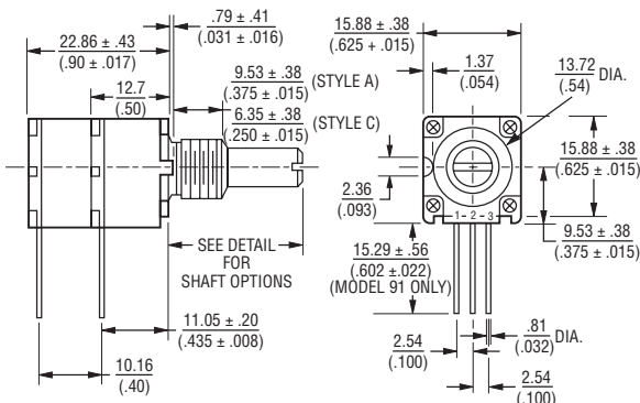
Model 93 PC Pin Terminals, "L" Pattern
