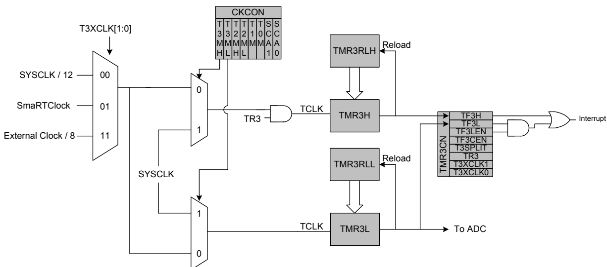
33.3.3. SmaRTClock/External Oscillator Capture Mode
