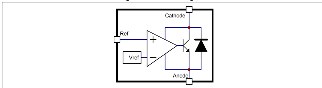
Figure 5. Block diagram
