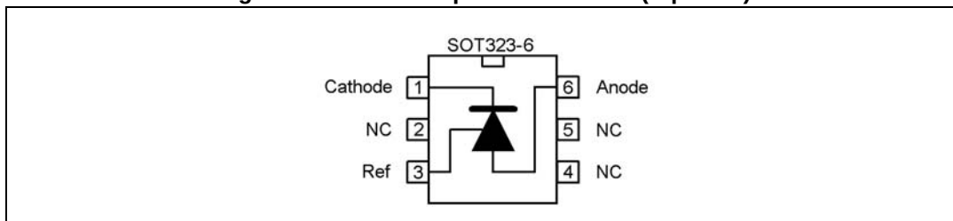
Figure 4. SOT323-6L pin connections (top view)
