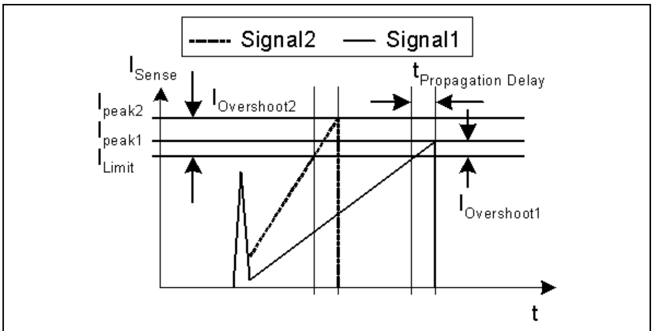
Figure 20 Current Limiting
