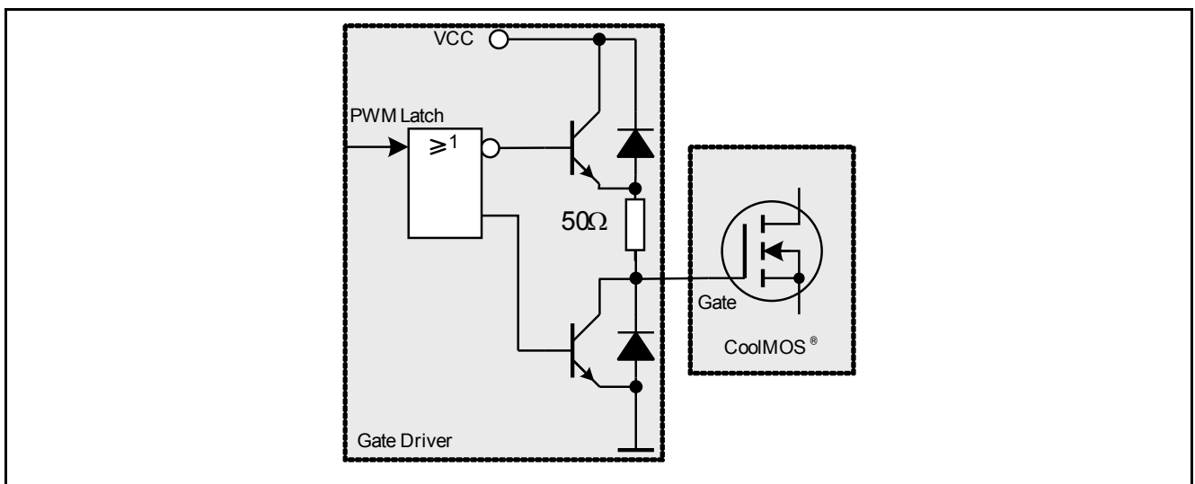
Figure 16 Gate Driver
