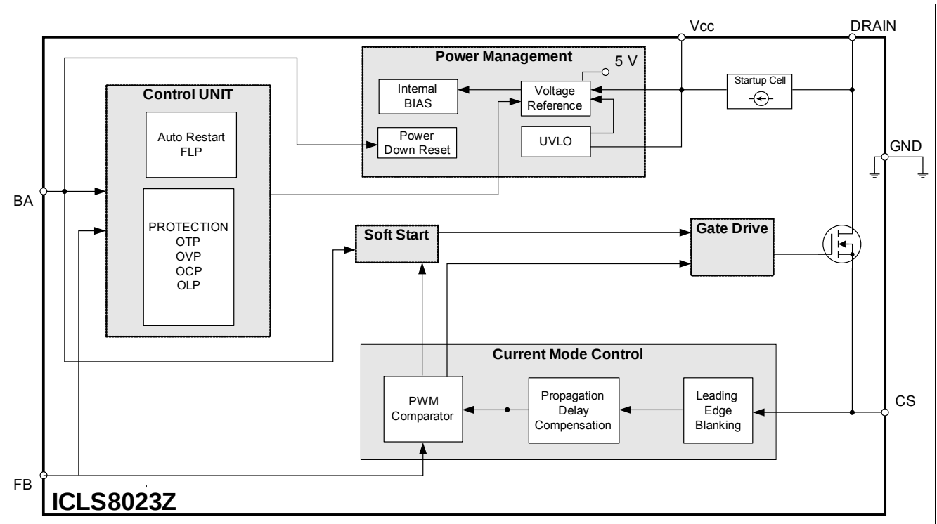
Figure 3 Block diagram of ICLS8023Z controllers
