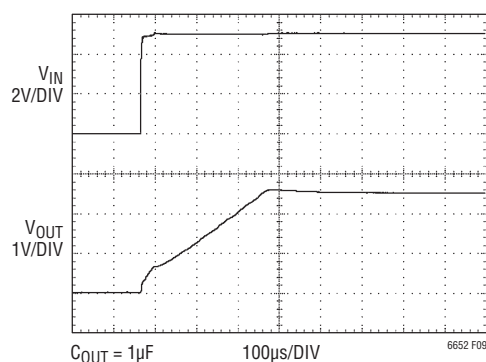
Figure 9. Start-Up Response with 1µF Output Capacitor
