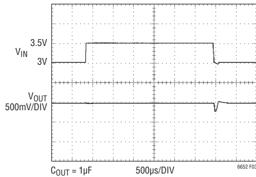
Figure 3. Transient Response with 1μF Output Capacitor
