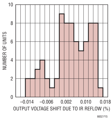
Figure 15. Output Voltage Shift Due to IR Reflow
