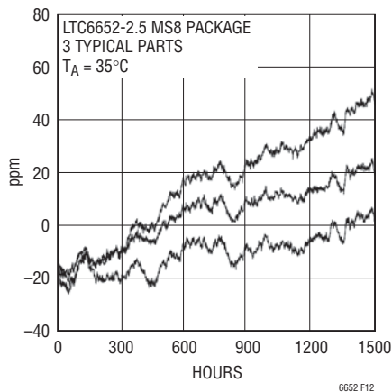
Figure 12. Long-Term Drift
