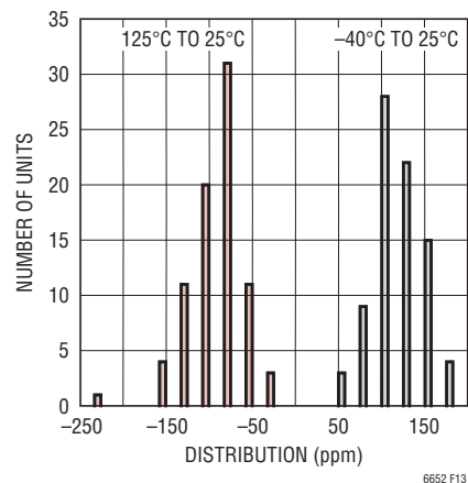
Figure 13. Hysteresis Plot -40^{\circ}\text{C} to 125^{\circ}\text{C}
