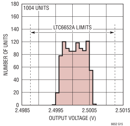
Typical V_{OUT} Distribution for LTC6652-2.5
