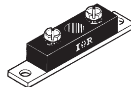
TO-244AB
