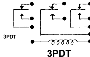
Triple Pole, Double Throw Relays.
