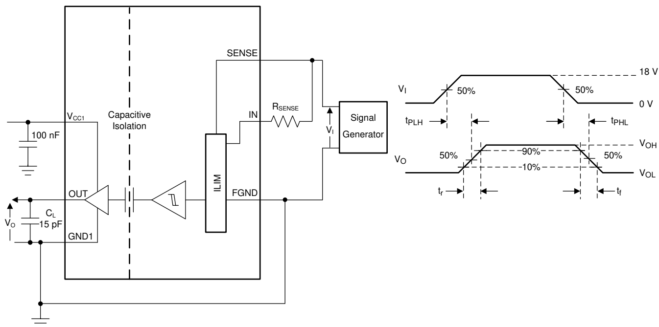
Figure 10. Switching Characteristics Test Circuit and Voltage Waveforms
