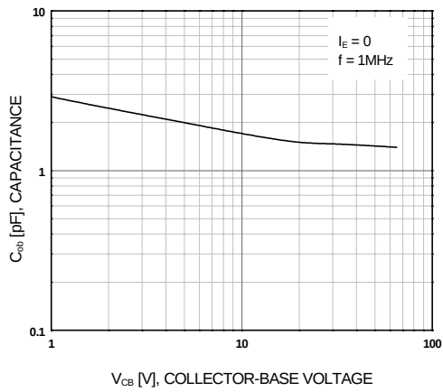
Figure 3. Output Capacitance
