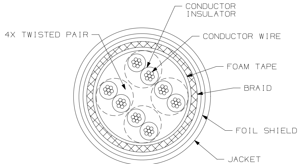
CROSS-SECTIONAL VIEW OF CABLE
