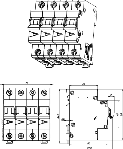
3+N-pole, 4-pole
