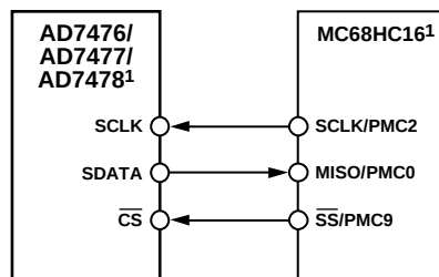
Figure 29. Interfacing to the MC68HC16
